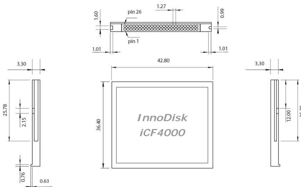
Figure 1: Mechanical Dimension of iCF4000
